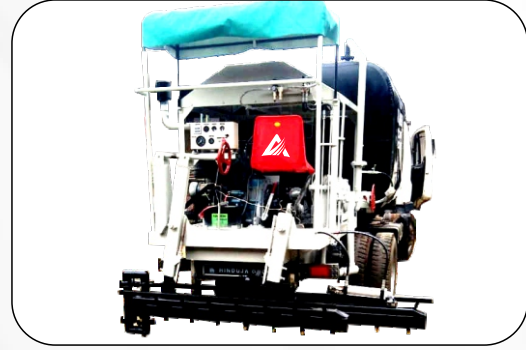
Truck Mounted Sprayer
